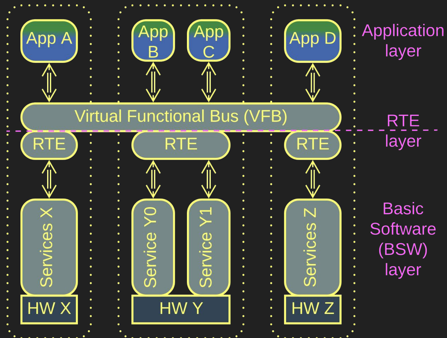
Automotive SOA
