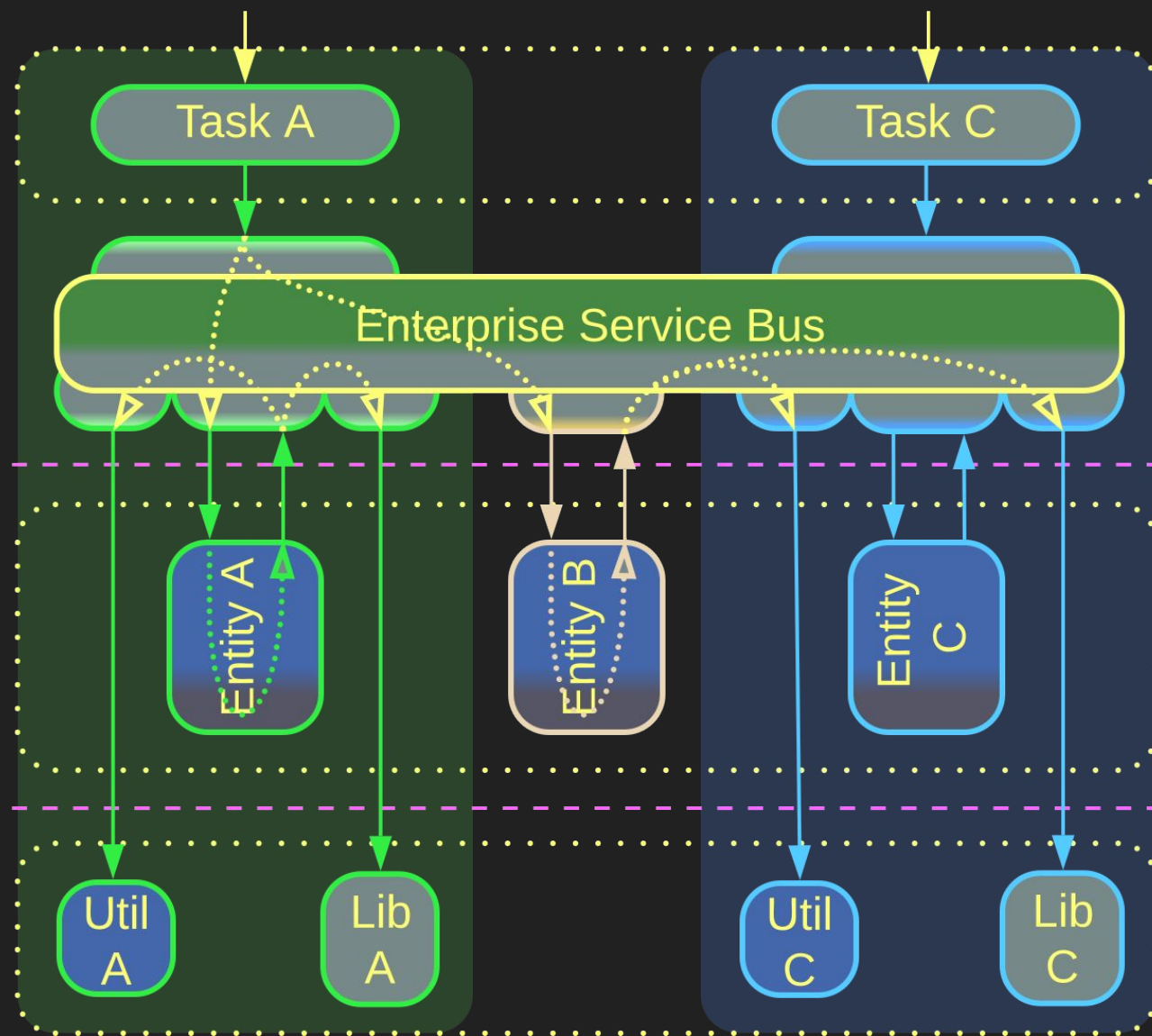
Enterprise SOA
