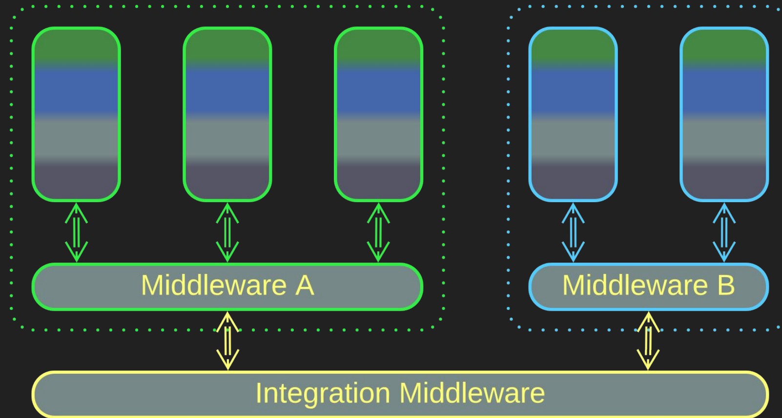
Bottom-Up Hierarchy
