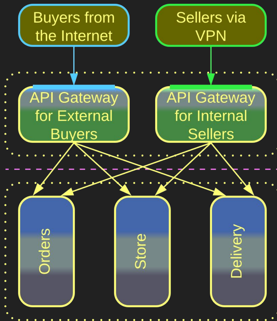
API Gateways
