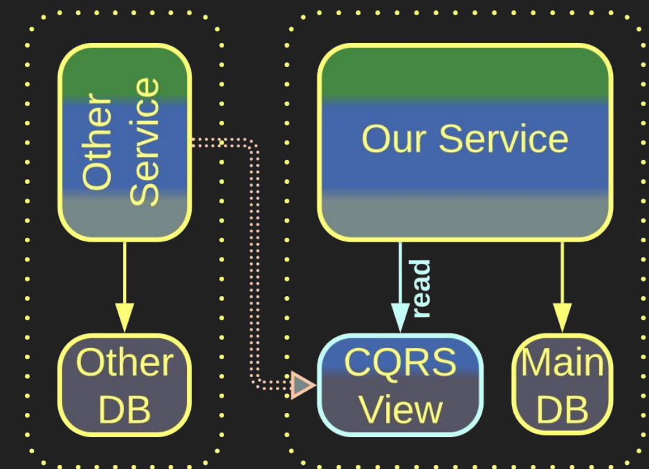
CQRS View
