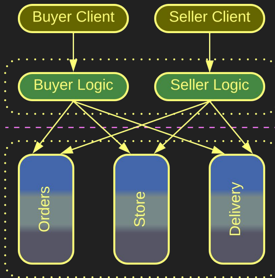
Orchestrators
