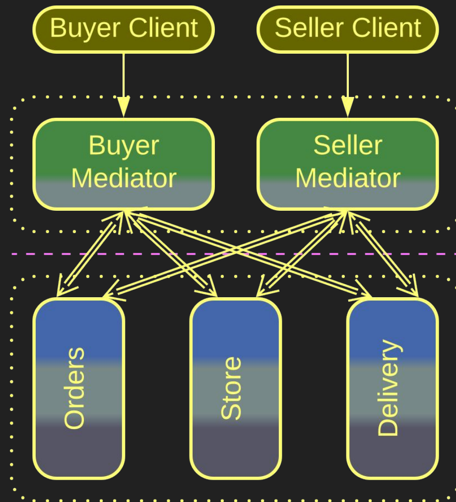
Event Mediators
