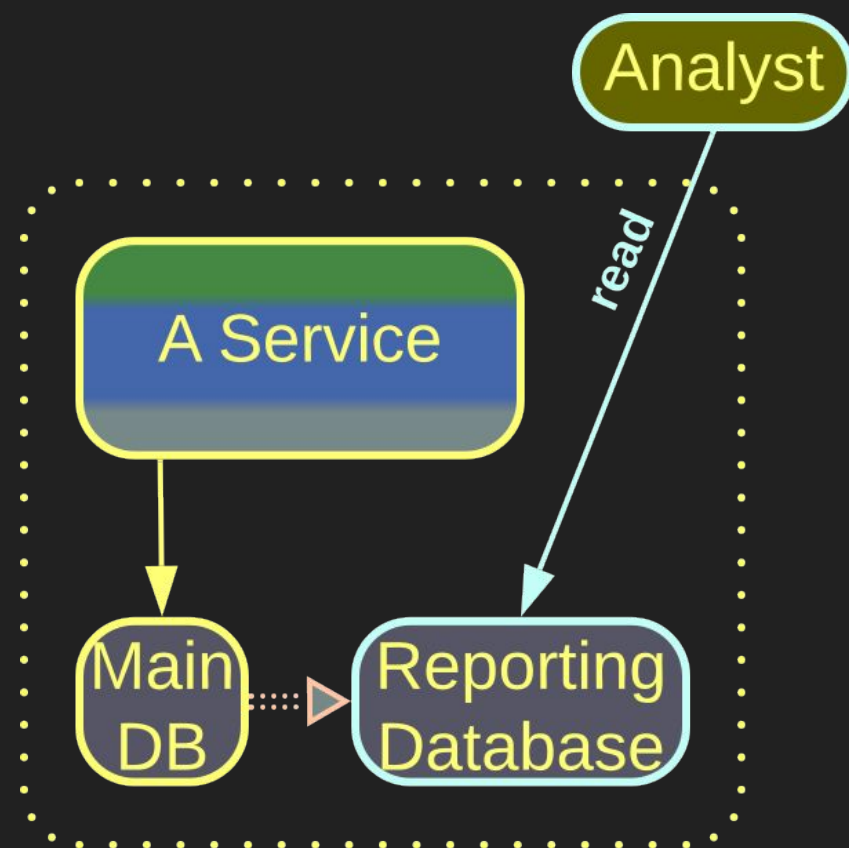
Reporting Database
